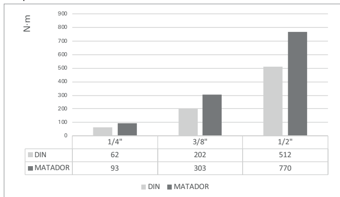
Torque test:
