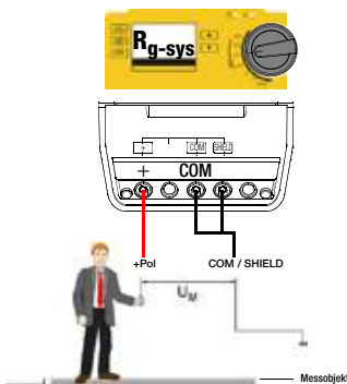
Measurement: R_{G\text{-system}} Personal bleeder resistance (human/shoes/flooring) to protective earth
